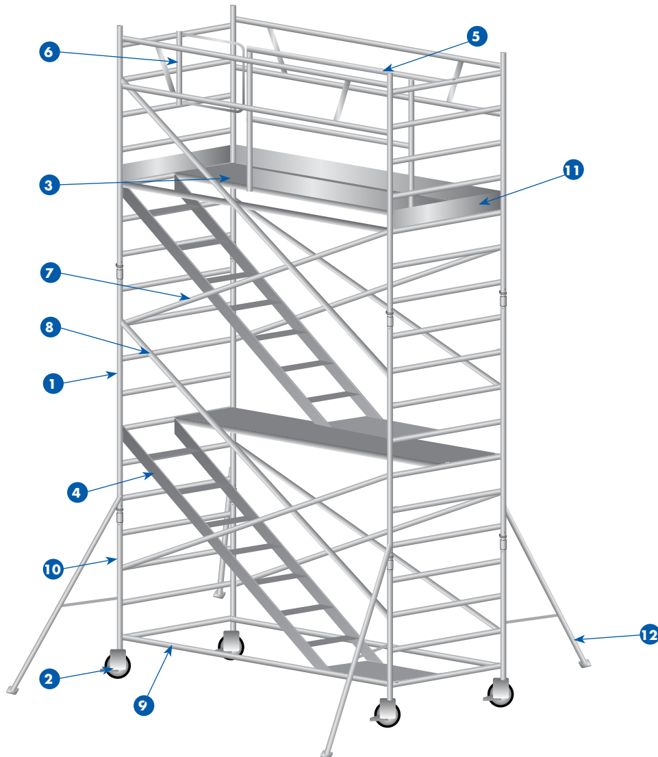
RS135-400-comfort
